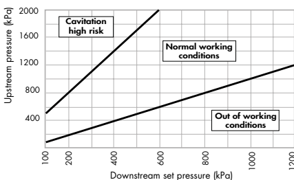
Cavitation diagram
